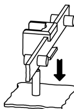
2. Assemble the flat rod guide onto the weld stud.
